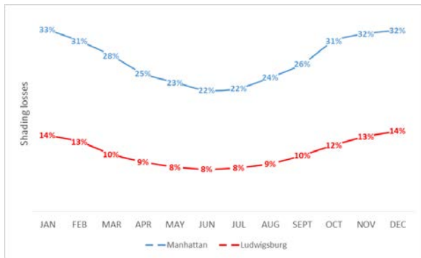
Figure 5: Rooftop monthly shading factors.
